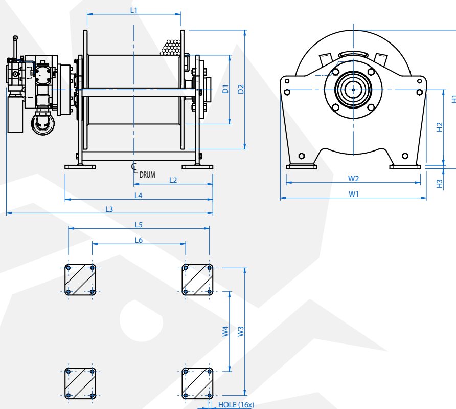
FOOTPRINT - TOP VIEW - A-A
