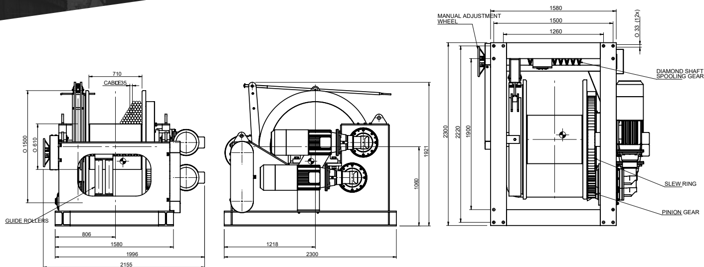
SRM25 E2 Drawing - Others available on request
