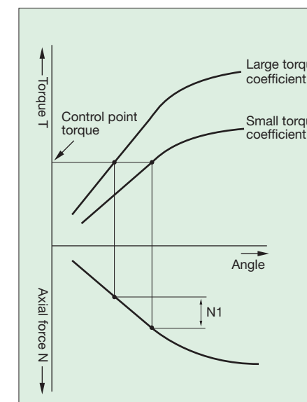
Torque Control
