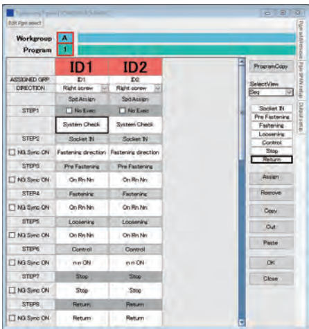
MU50 Fastening Program Menu
