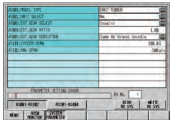
AXIS Unit System Setting
